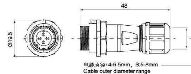
In-line cable connector PS(Reverse Cable Socket)RP(Reverse Cable Plug)Series 电缆对接插座
