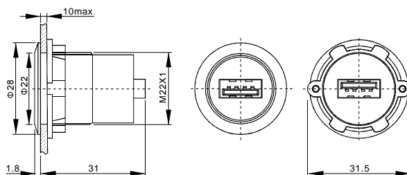
产品描述 : USB2.0 头部A型母/尾部A型母 Product Description: USB2.0 HEAD FEMALE A/BACK FEMALE A
