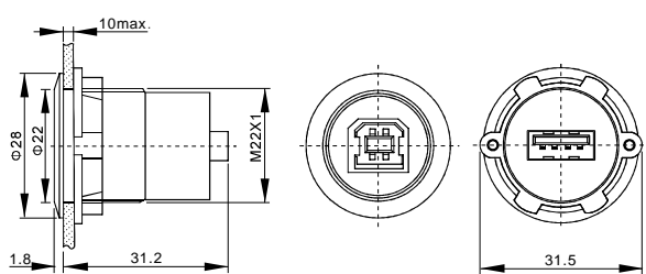
产品描述 : USB2.0 头部B型母/尾部A型母 Product Description: USB2.0 HEAD FEMALE B/BACK FEMALE A
