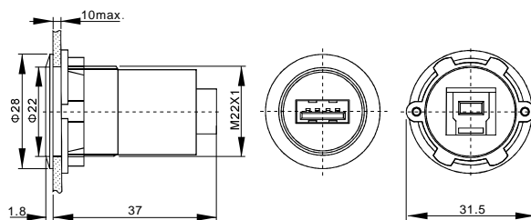
产品描述 : USB3.0 头部A型母/尾部B型母 Product Description: USB3.0 HEAD FEMALE A/BACK FEMALE B
