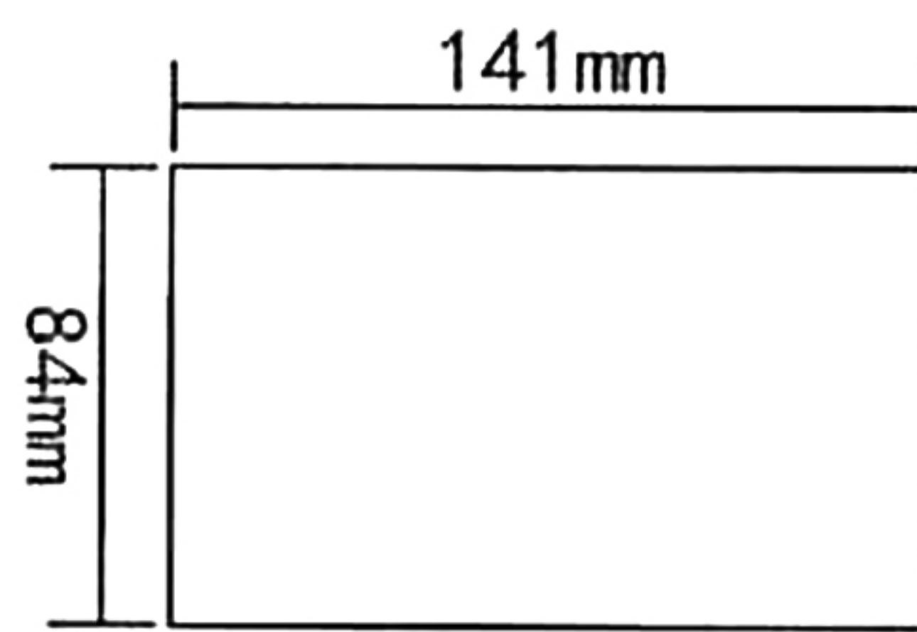
Cut-out
